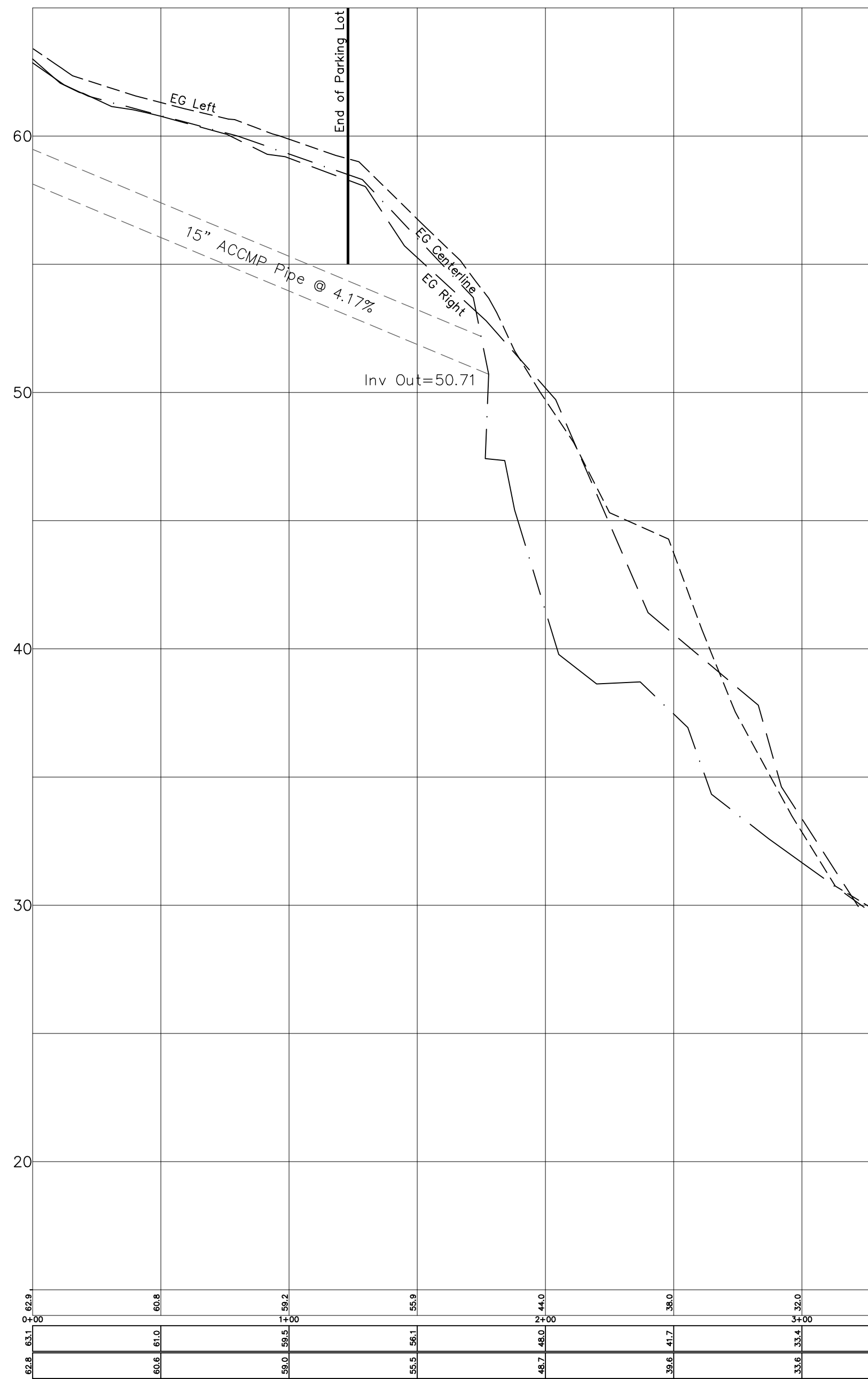
EXITING PROFILE ALONG DITCH 1"=40' H 1"=4' V
