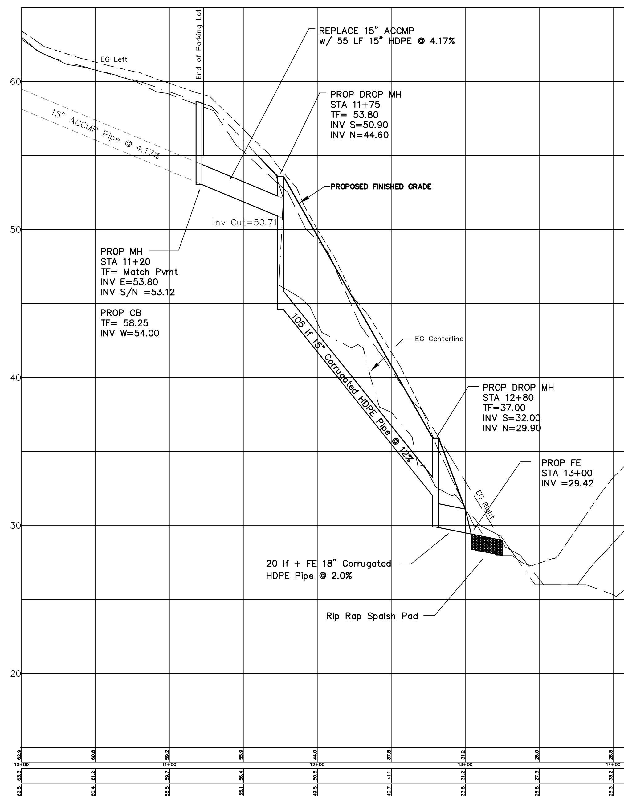
EXITING/PROPOSED PROFILE ALONG PROPOSED PIPE 1"=40' H 1"=4' V
